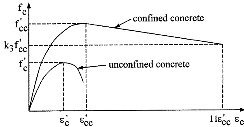
Fig. 4 Equivalent uniaxial stress-strain curve for concrete
