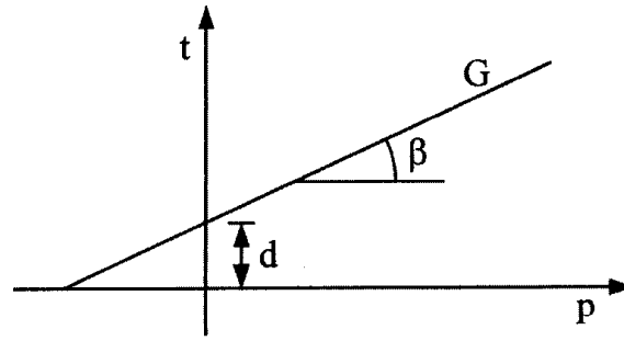
Fig. 5 Linear Drucker-Prager yield criterion for concrete
