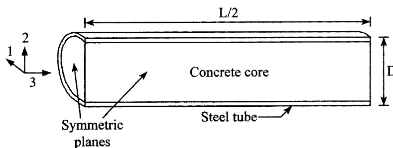
Fig. 7 Conceptual sketch and finite element modeling of CFT column
