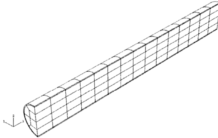
Fig. 8 Finite element mesh for CFT columns
