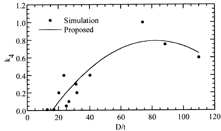
Fig. 12 k_4 versus D/t for CFT columns
