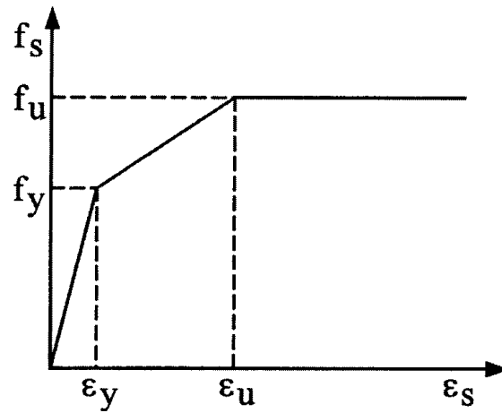
Fig. 2 Bilinear stress-strain curve of steel
