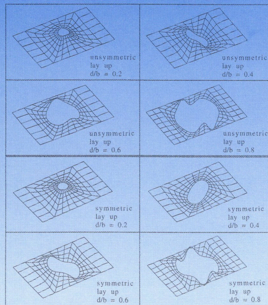
Fig. 12 Buckling modes of clamped [(\pm\theta_1/90/0)_2/(0/90/\mp\theta_2)_2] and [\pm\theta/90/0]_2 composite plates with combined inplane and lateral loads, with circular cutouts and under optimal fiber orientations ( a/b=1.5 )
